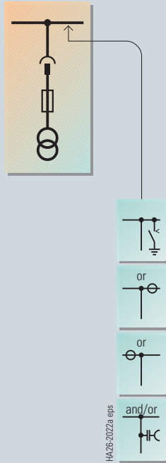
Metering panel
